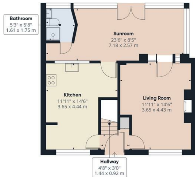
Floor 0 Building 1
